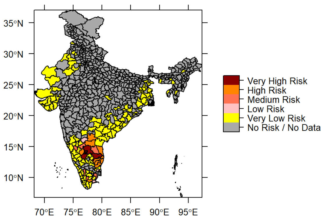
Risk Prediction of Anthrax for the month of January 2019
